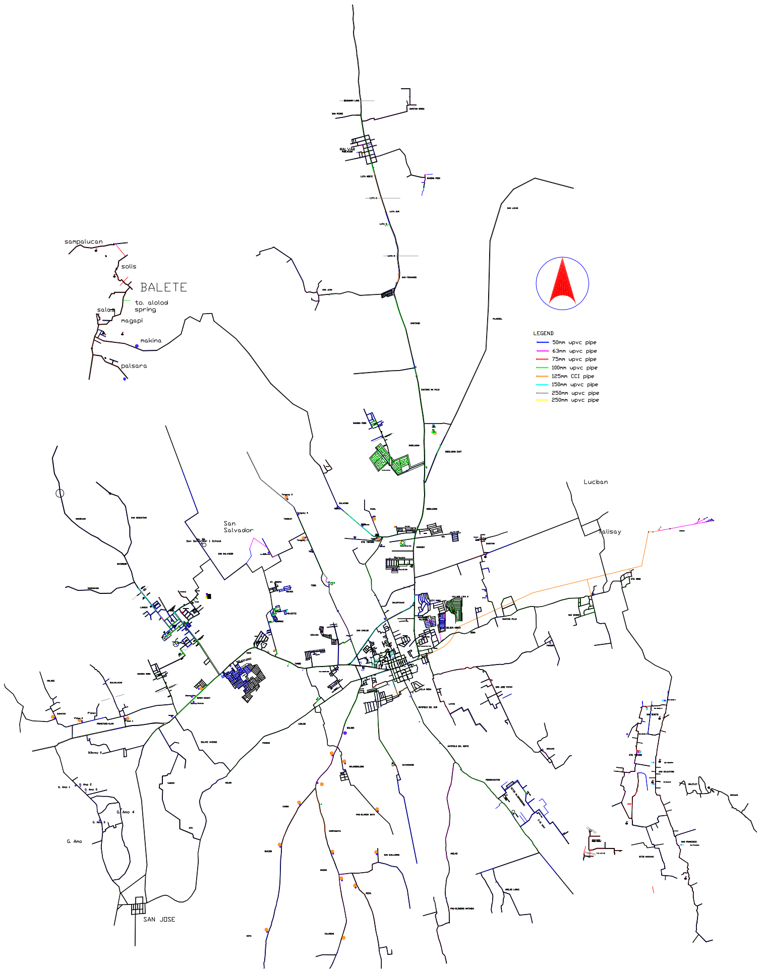
METRO LIPA WATER DISTRICTS' SERVICE AREA
